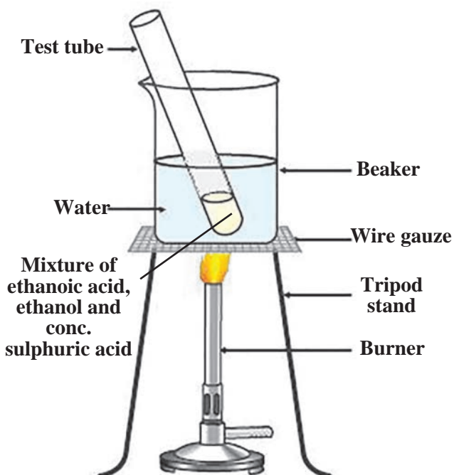
9.25 Esterification Reaction
