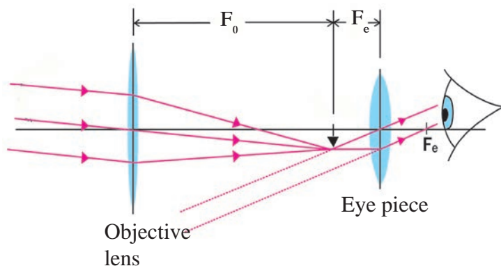
7.18 Refracting telescope
